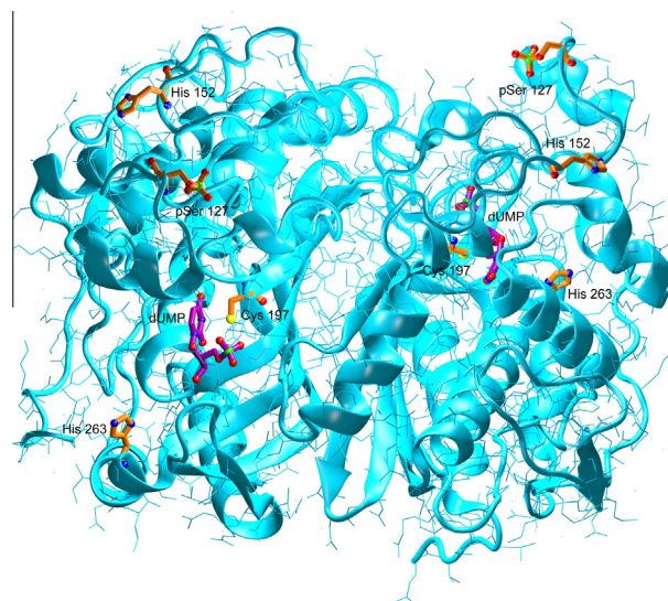
Fig. 2. Crystal structure of the dimeric \text{CepTS} -dUMP complex. dUMP, catalytic Cys197, His152, His263 and pSer127 are shown as licorice and labelled. Carbon atoms are orange or violet (dUMP), and oxygen, nitrogen, phosphorus and sulfur atoms are red, blue, green and yellow, respectively. This figure was prepared with VMD [27] and rendered with Raster3D [28].
